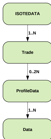
Figure 8 Figure 10 Scheme of order structure
