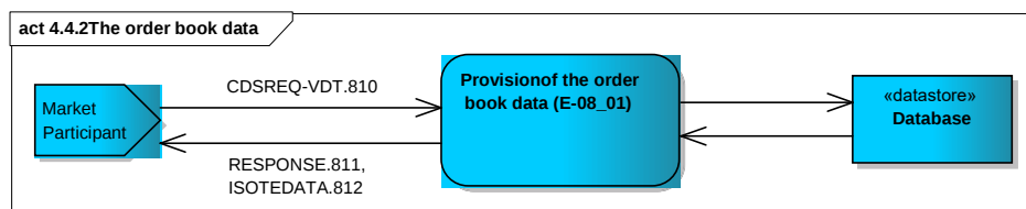
Figure 22 Figure 24 Provision of order book data scheme
