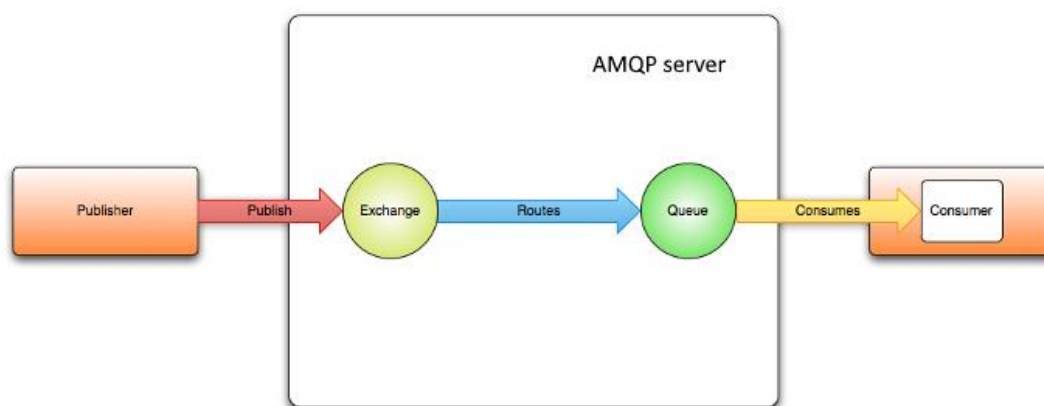
Figure 6 Figure 8 AMQP communication concept
