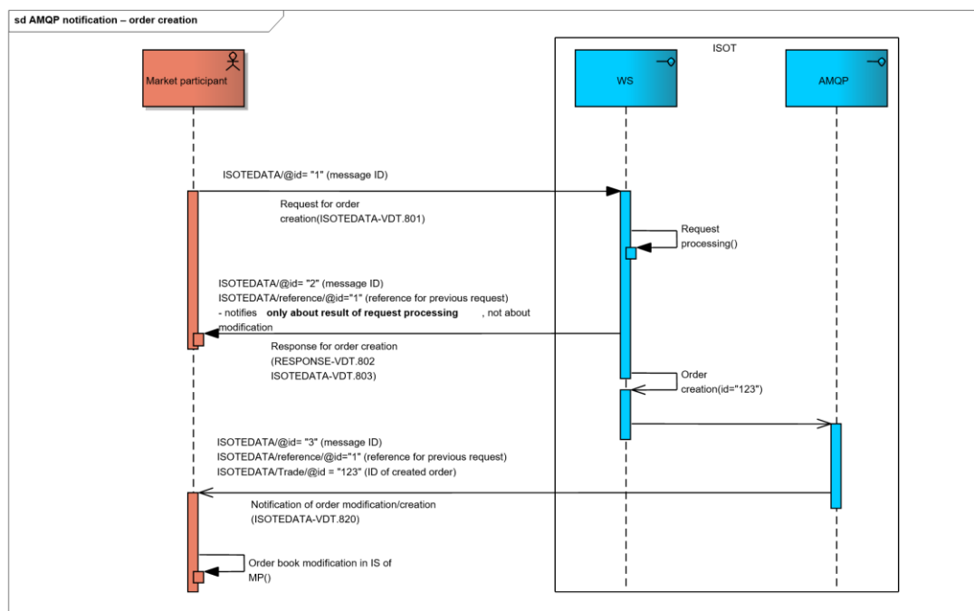
Figure 30 Figure 33 Order of send messages scheme – order creation (AMQP notification)
