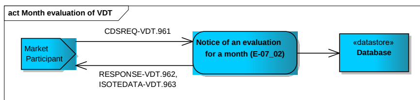
Figure 27 Figure 30 Notice of an evaluation for a month scheme
