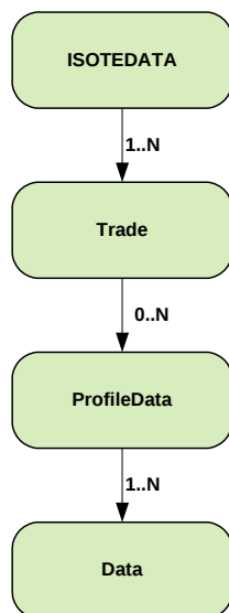
Figure 9 Figure 11 DM results structure scheme
