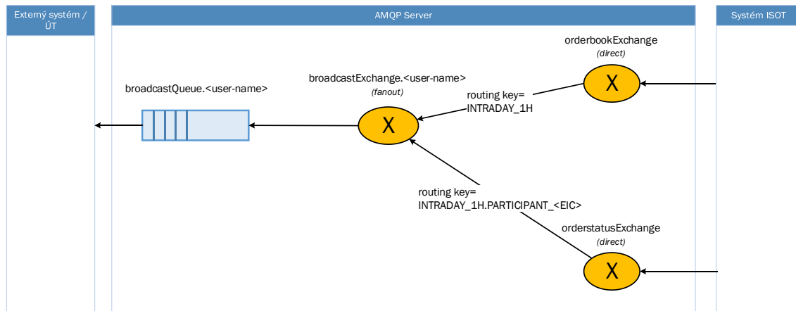
Figure 7 Figure 9 Scheme of notification messages flow on intraday market
