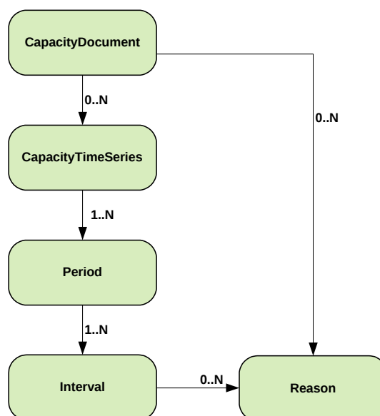
Figure 37 Figure 40 Schema of CapacityDocument structure
