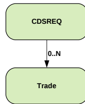
Figure 14 Figure 16 Scheme of CDSRWQ-VDT structure
