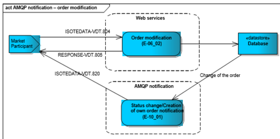
Figure 31 Figure 34 Sending messages scheme – order modification (AMQP notification)
