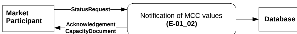
Figure 35 Figure 38 Notification schema of MCC values
