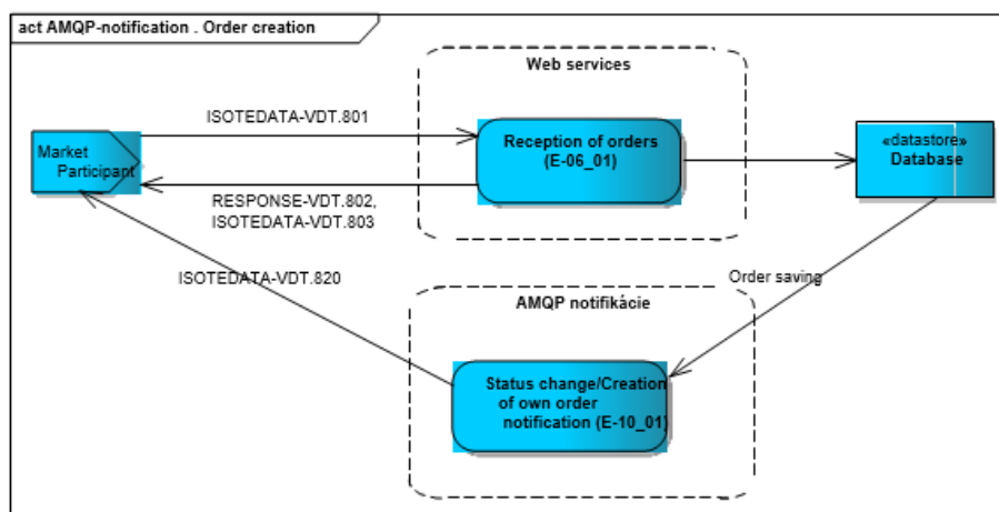
Figure 29 Figure 32 Sending messages scheme – order creation (AMQP notification)
