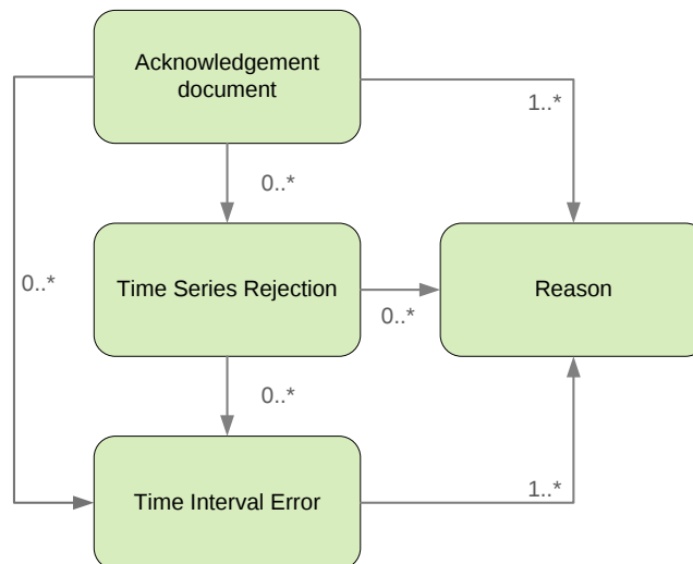
Figure 36 Figure 39 Scheme of Acknowledgement structure
