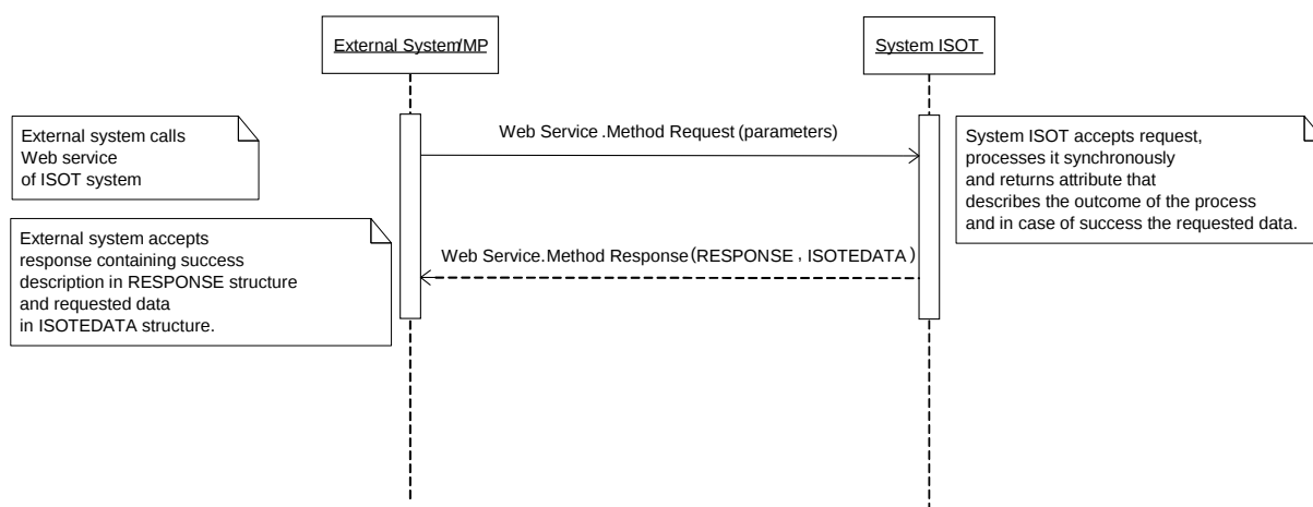
Figure 5 Figure 7 The principle of synchronous communication.
