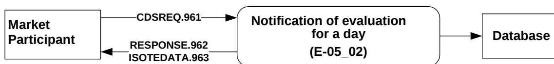
Figure 28 Notification schema of evaluations for day for market participant
