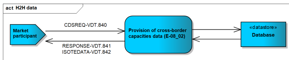
Figure 25 Provision of cross-border capacities scheme
