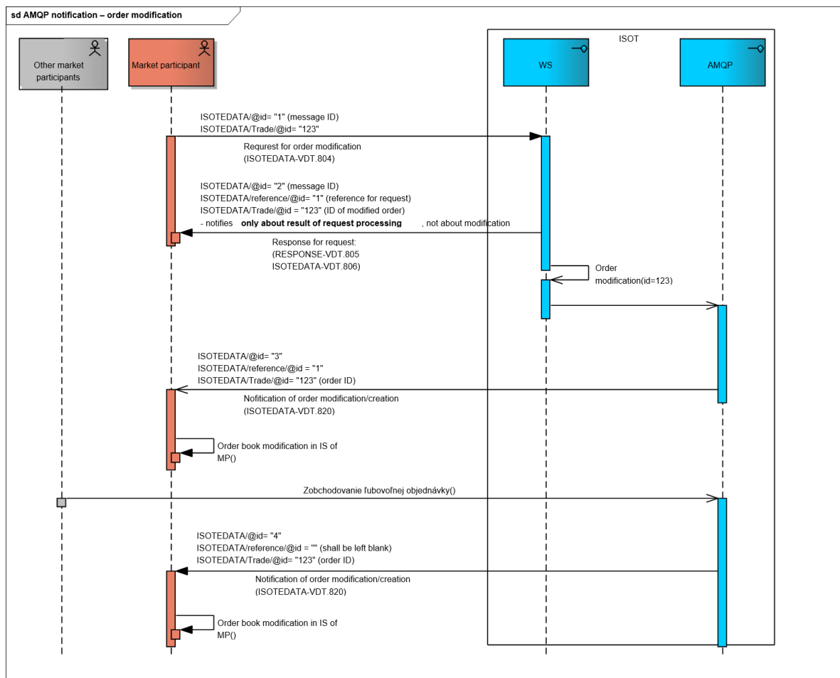
Figure 32 Figure 35 Order of sent messages scheme – order modification (AMQP notification)
